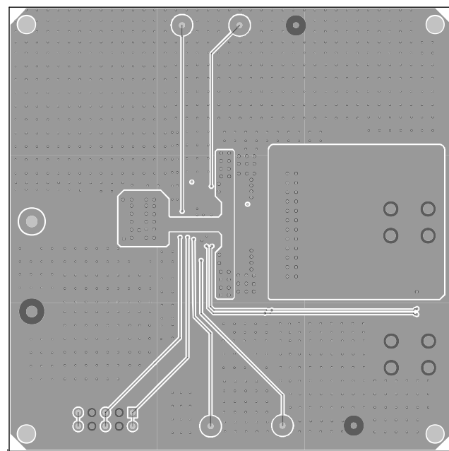
Figure 6: Mid-Layer 2
