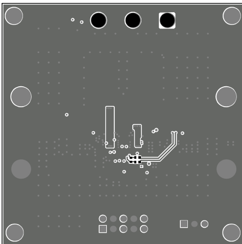
Figure 7: Bottom Layer
