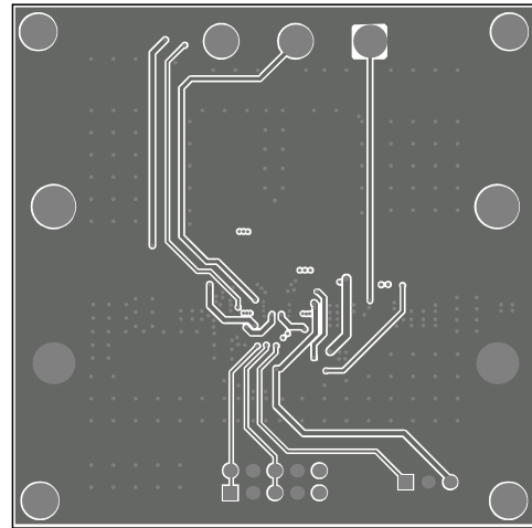
Figure 6: Mid-Layer 2
