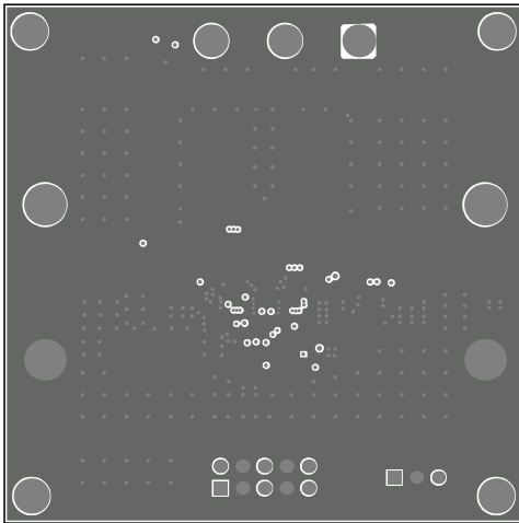
Figure 5: Mid-Layer 1
