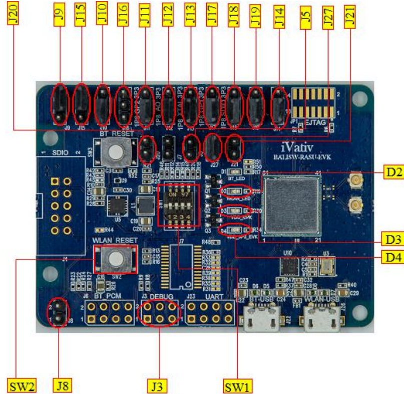
Figure 1: EVIA USB EVK
