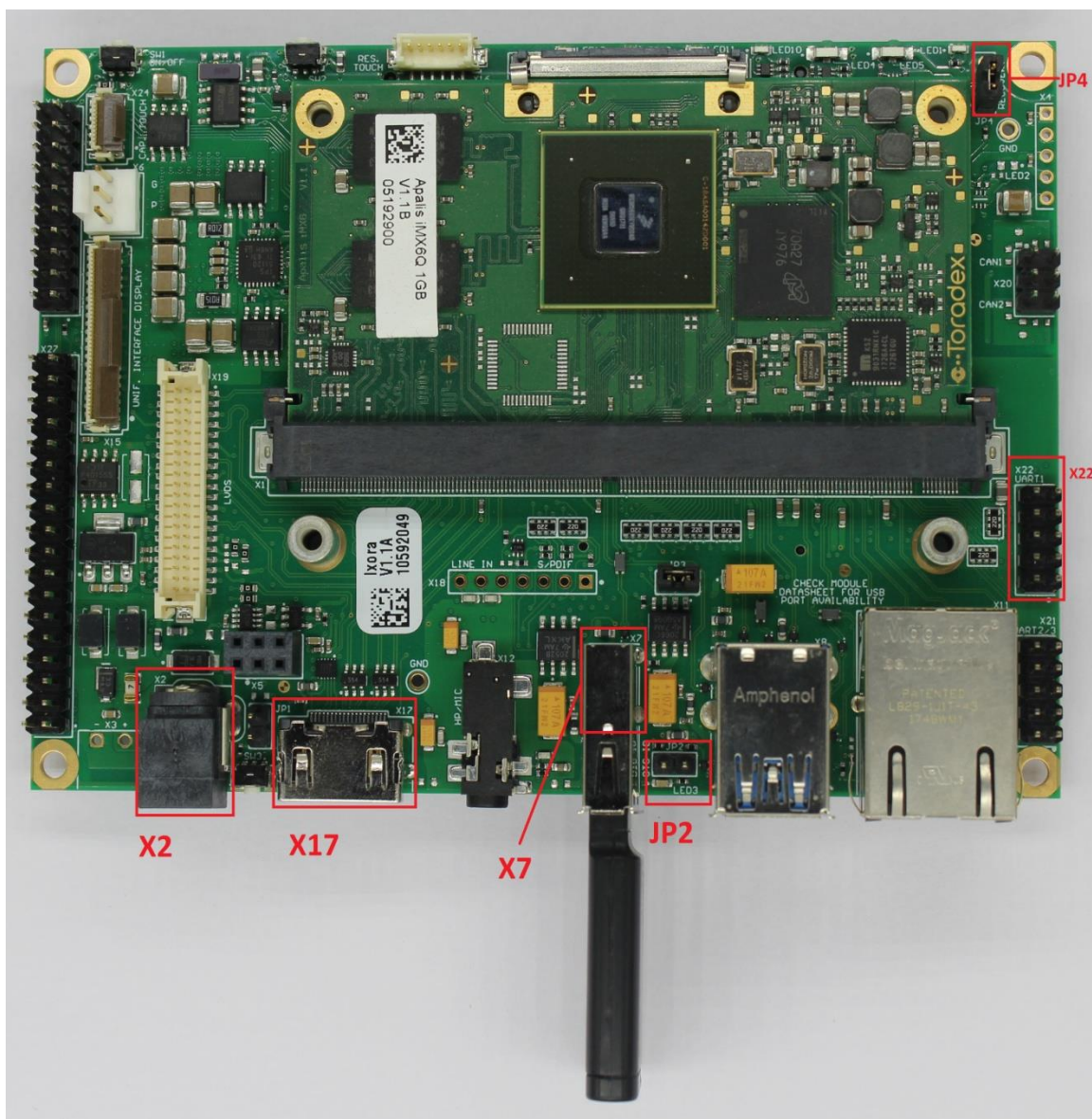
Figure 13: Recovery mode setup on Ixora
