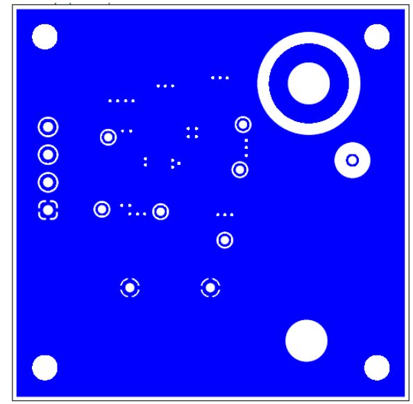
Figure 10. FAD1110EVB PCB Internal Plane 2 Drawing
