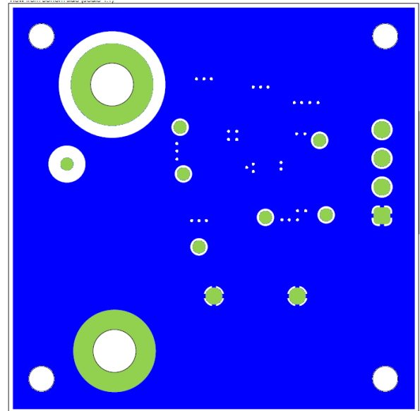
Figure 8. FAD1110EVB PCB Bottom Composite Drawing (bottom view)
