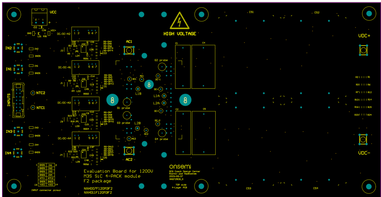
Figure 24. Assembly TOP
