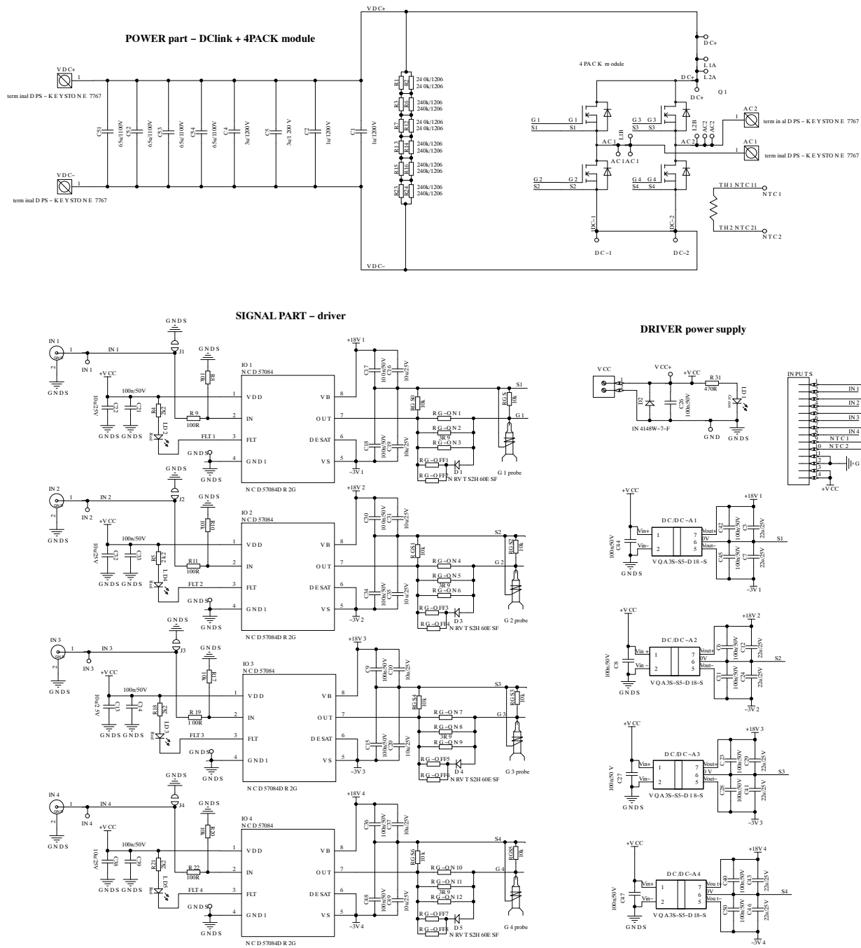
Figure 19. Complete Schematics
