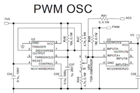
Figure 7. PWM Generator Schematic
