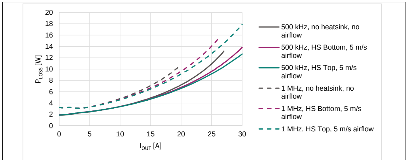
Figure 25 Example power loss results with Vishay IHLP7575-JZ 3.3 \mu H inductor
