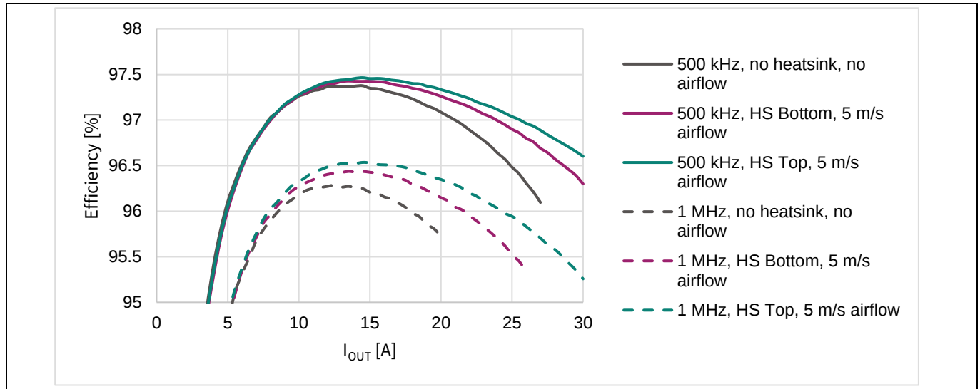
Figure 24 Example efficiency results with Vishay IHLP7575-JZ 3.3 \mu H inductor
