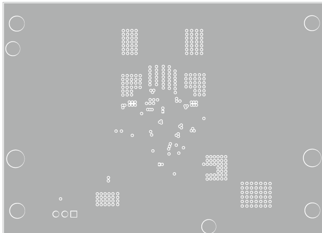
Figure 3: Middle Layer 1
