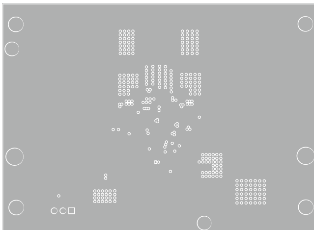
Figure 6: Middle Layer 4
