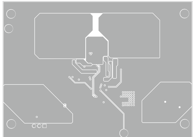
Figure 4: Middle Layer 2
