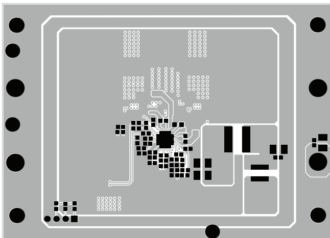
Figure 7: Bottom Layer
