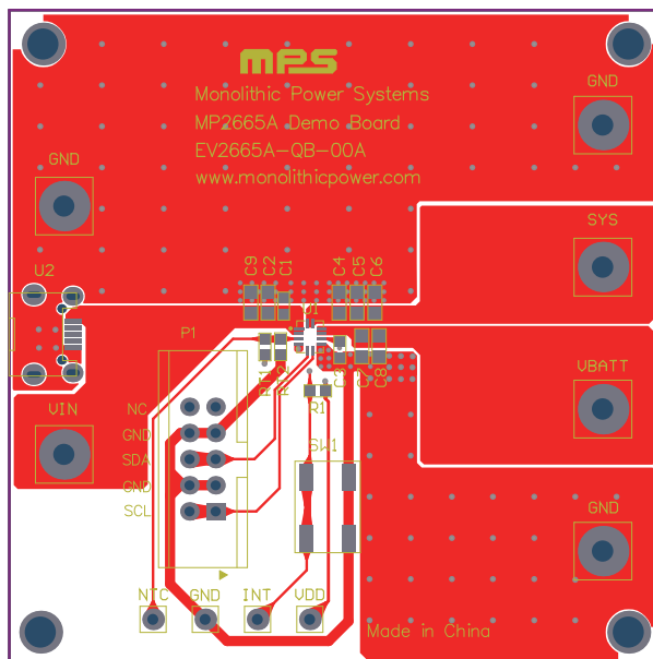
Figure 26: Top Layer
