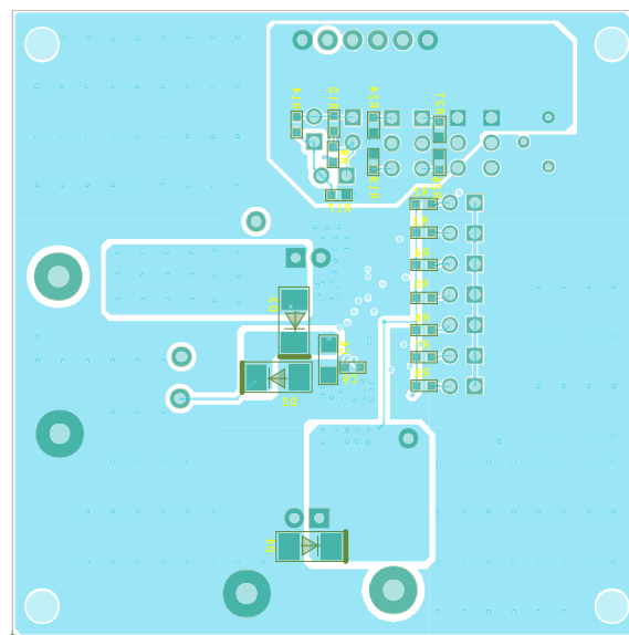
Figure 6: Bottom Layer
