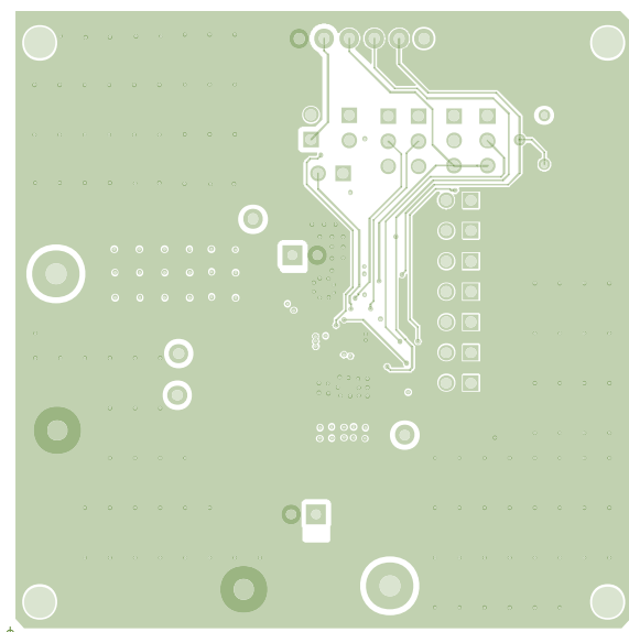
Figure 5: Mid-Layer 2
