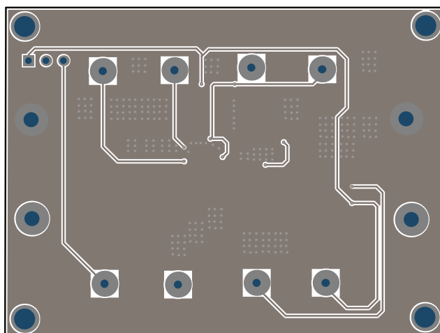
Figure 3: Bottom Layer
