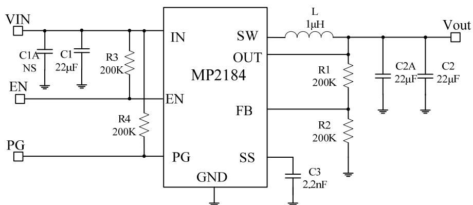
Figure 1—Typical Application Circuit for MP2184GTL
