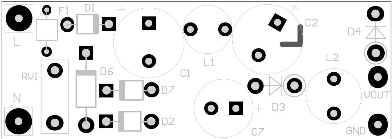
Figure 5: Top Layer
