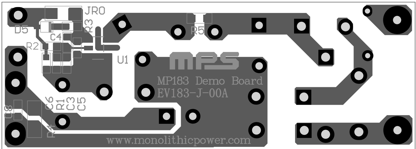
Figure 6: Bottom Layer
