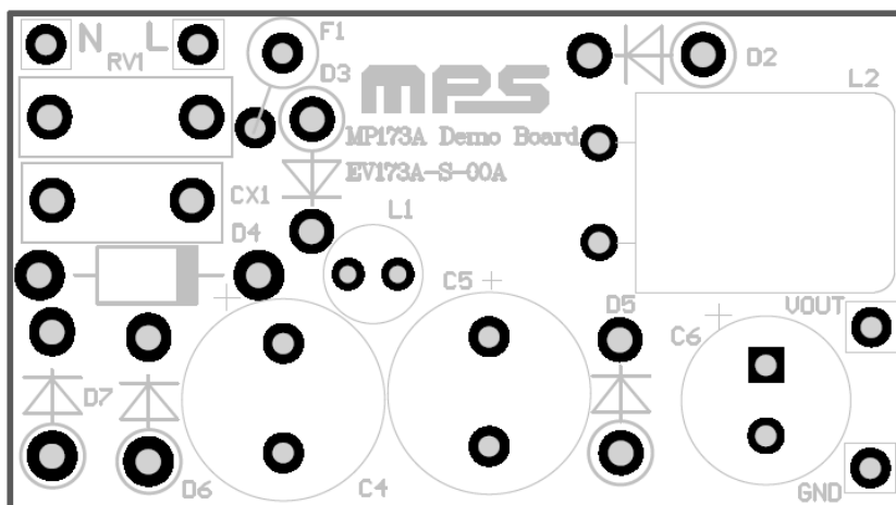
Figure 2: Top Layer
