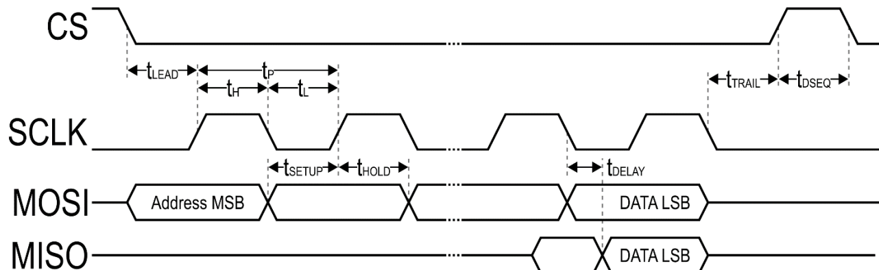
Figure 24 - SPI Slave Interface Timing
