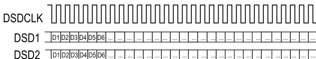
Figure 14 - DSD Format, 1-bit stream
