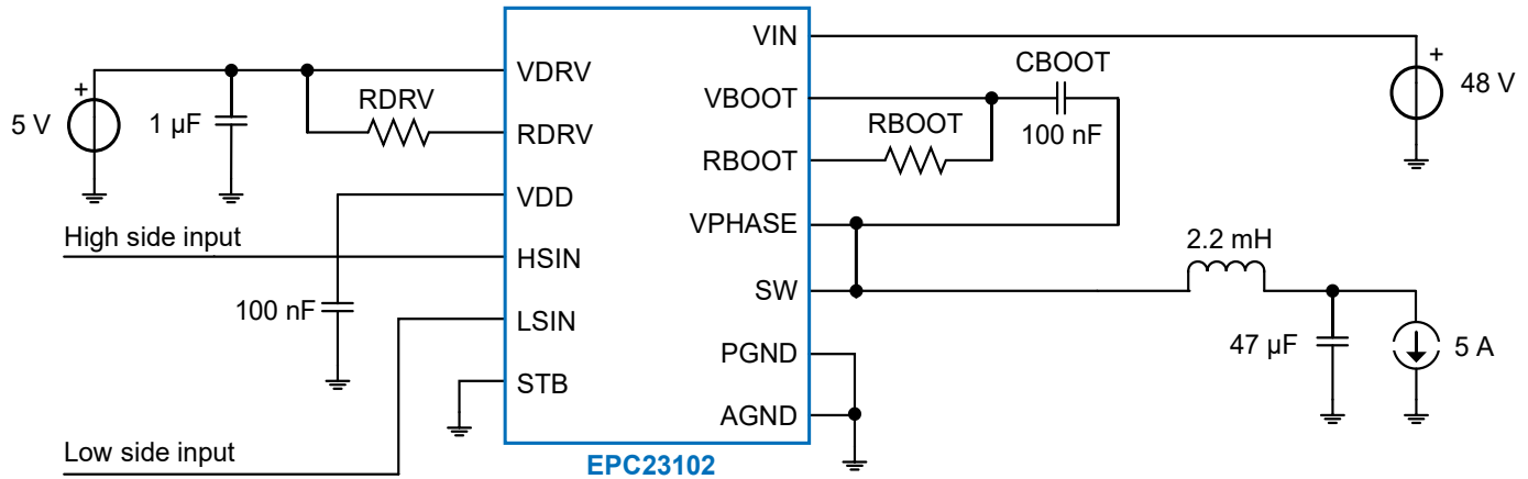
Figure 3a: Test Circuit for Dynamic Characteristics
