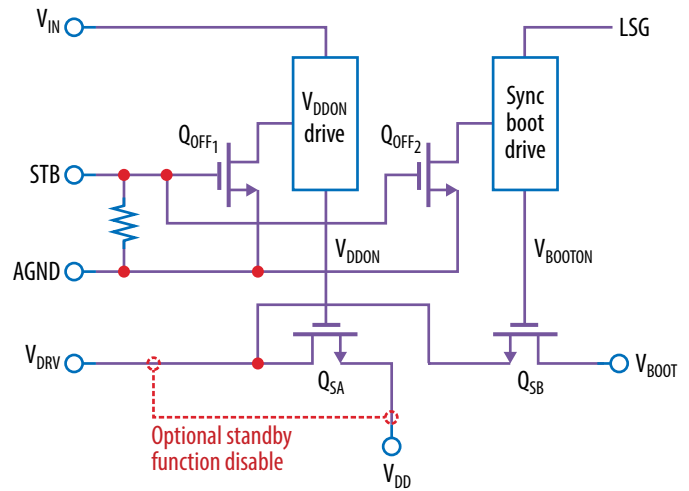
Figure 14: Simplified Circuit Diagram of V IN , V DRV , V DD , and V BOOT Power Supplies
