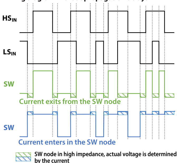
Figure 18: EPC23102 Input-to-Output Timing Diagram
