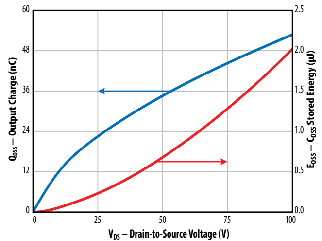
Figure 5b: EPC23102 LS Typical Output Charge and C_{OSS} Stored Energy
