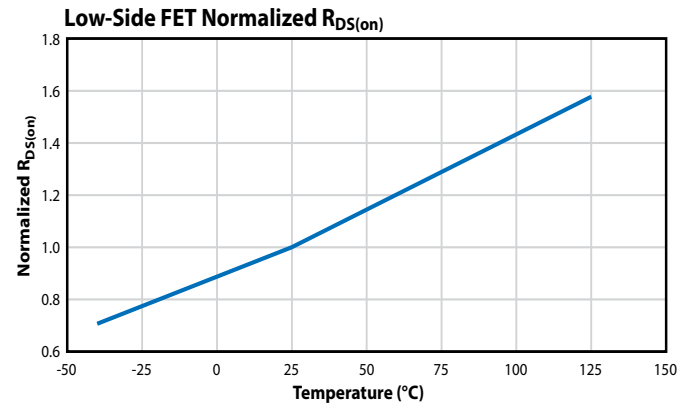
Figure 6b: Low Side FET Normalized R_{DS(on)}
