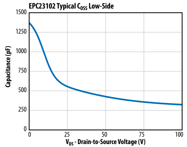
Figure 4b: C_{OSS\_LSFET} for low-side Power GaN FET
