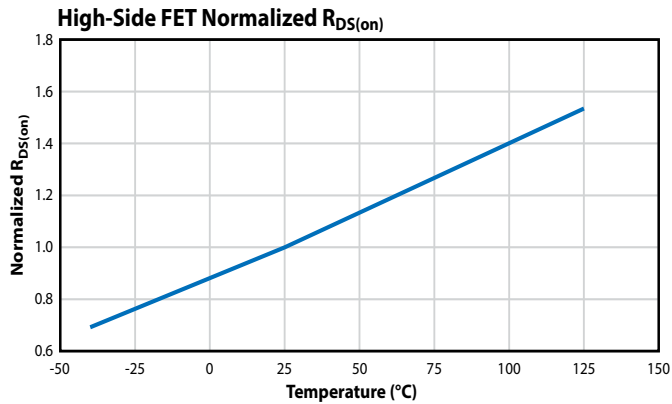
Figure 6a: High Side FET Normalized R_{DS(on)}
