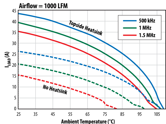
Figure 11: Thermal Derating Curves for Output Current Rating of EPC23102 IC using EPC90147 Evaluation Board
