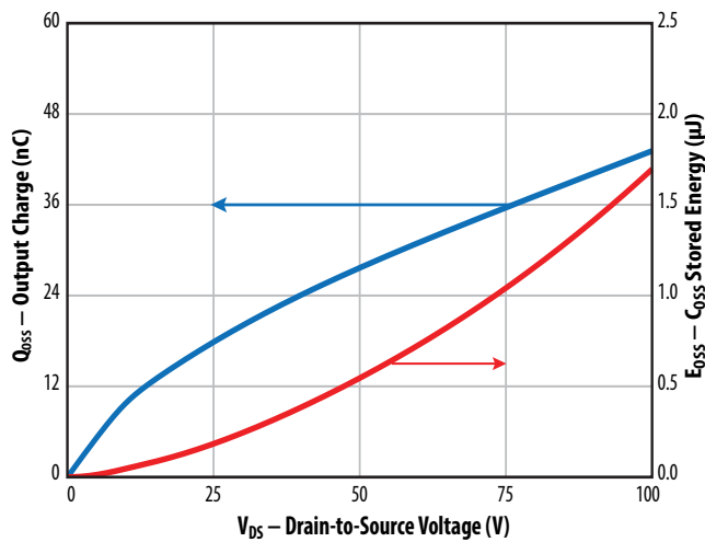
Figure 5a: EPC23102 HS Typical Output Charge and C_{OSS} Stored Energy
