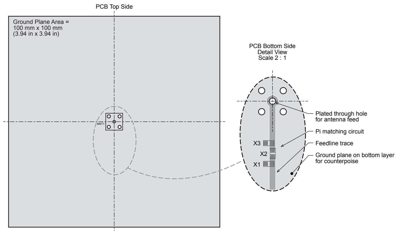
Figure 8. 2.4 GHz Vertical Helical Antenna Recommended Layout
