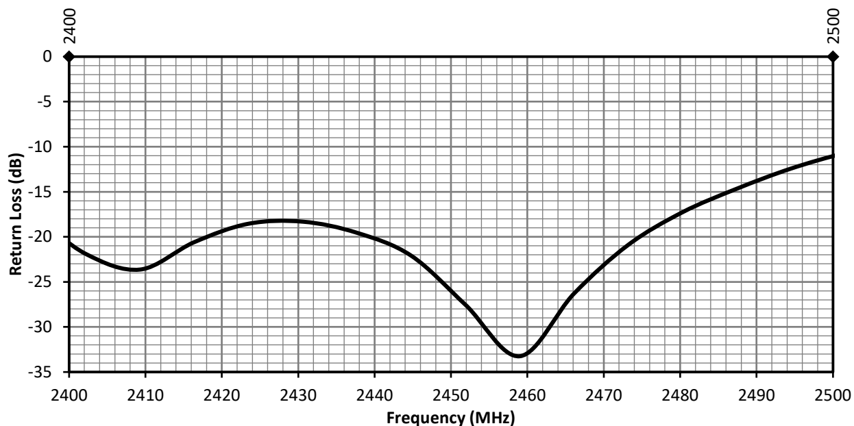
Figure 3. 2.4 GHz Vertical Helical Antenna Return Loss
