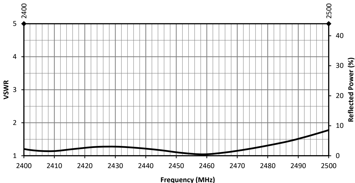
Figure 2. 2.4 GHz Vertical Helical Antenna VSWR
