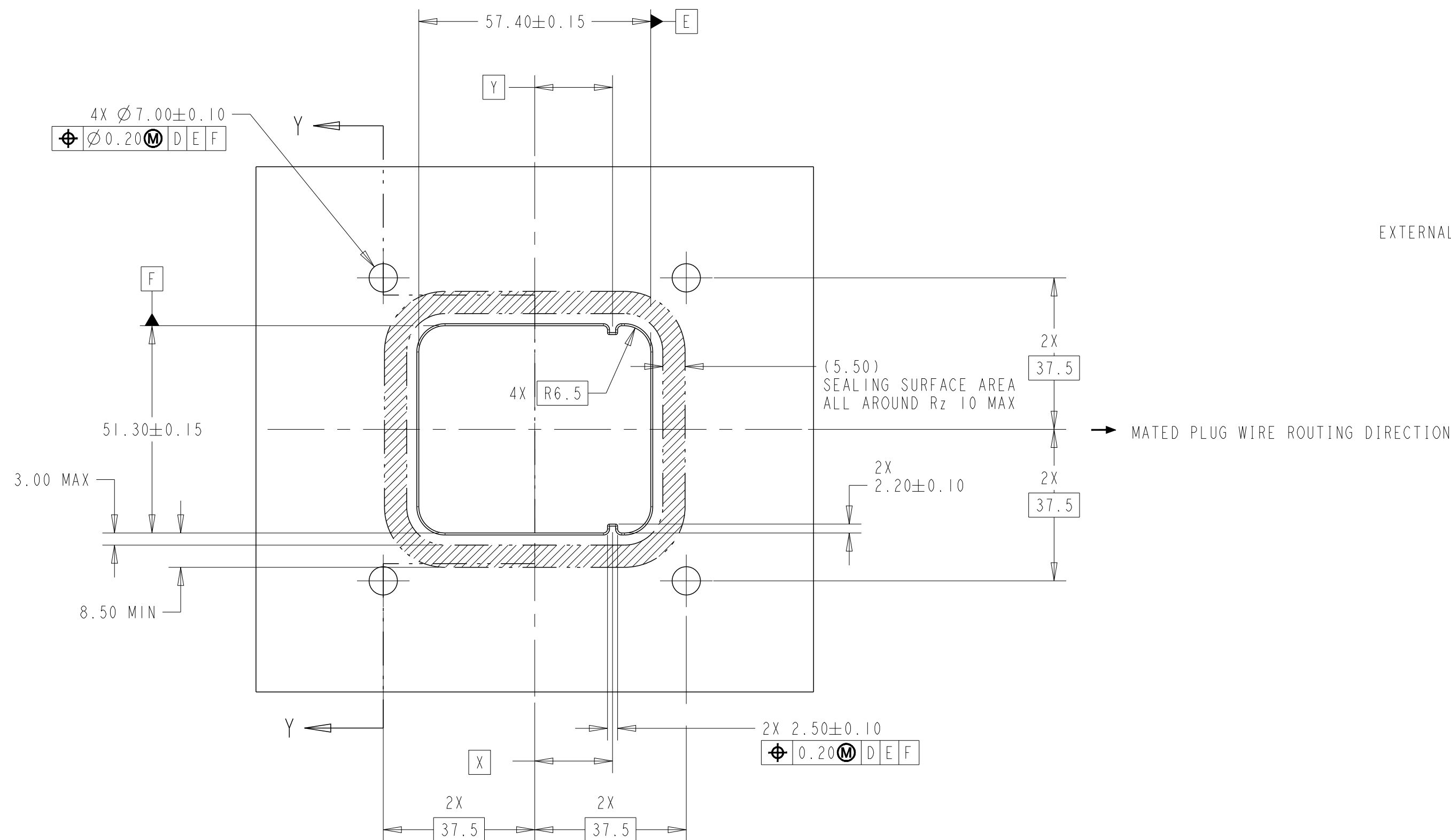
HEADER MOUNTING INTERFACE, TYPE-2 (CODE-A SHOWN)
