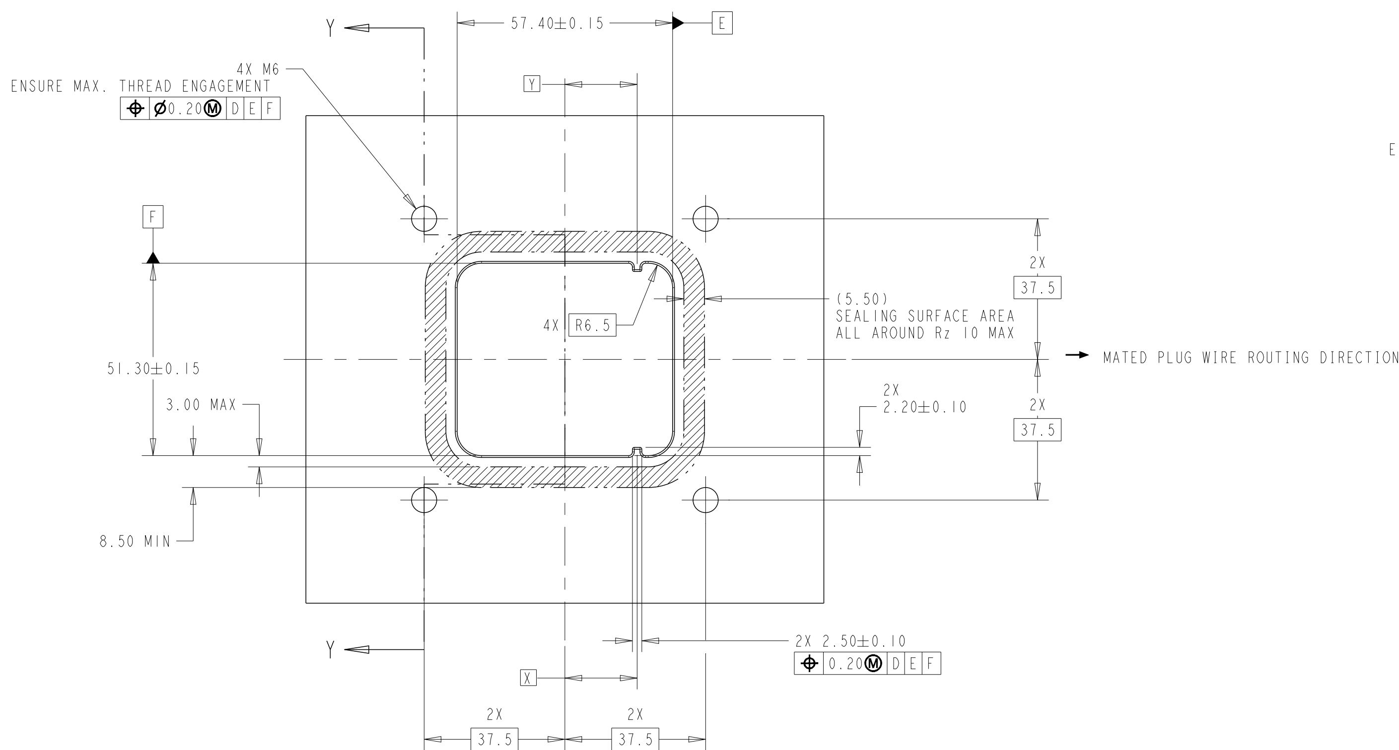
HEADER MOUNTING INTERFACE, TYPE-1 (CODE-A SHOWN)
