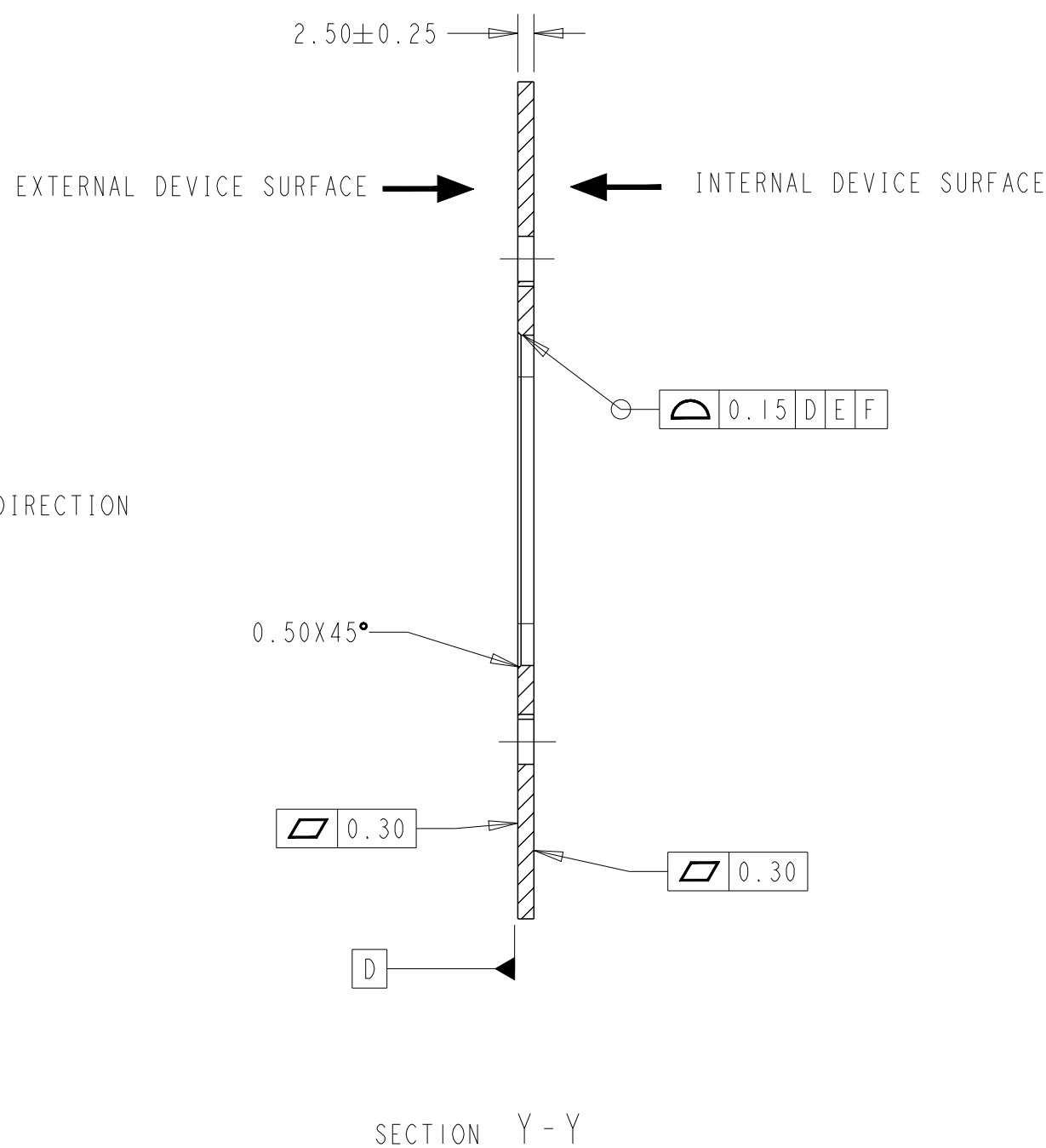
HEADER MOUNTING INTERFACE, TYPE-2 (CODE-A SHOWN)
