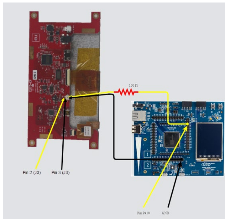
Figure 8. Renesas Synergy S7G2 Signal and Ground
