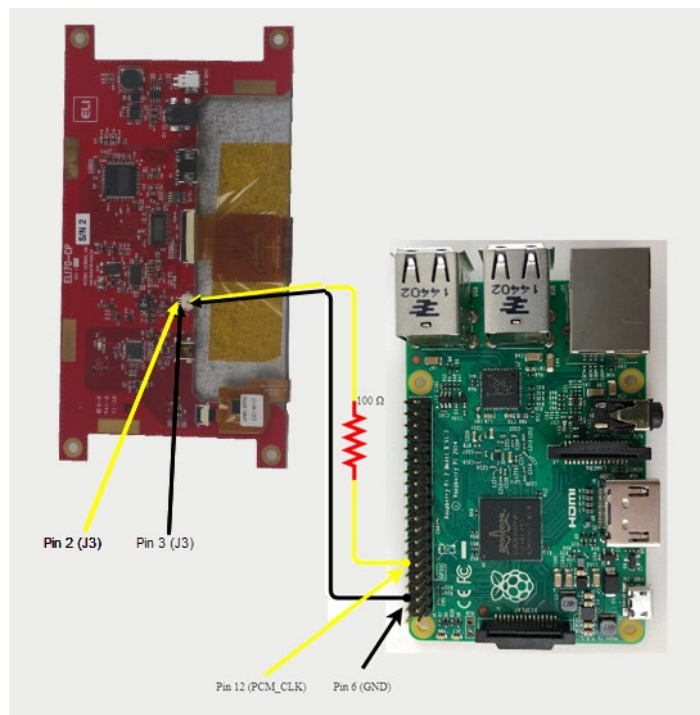
Figure 6. Raspberry Pi Signal and Ground
