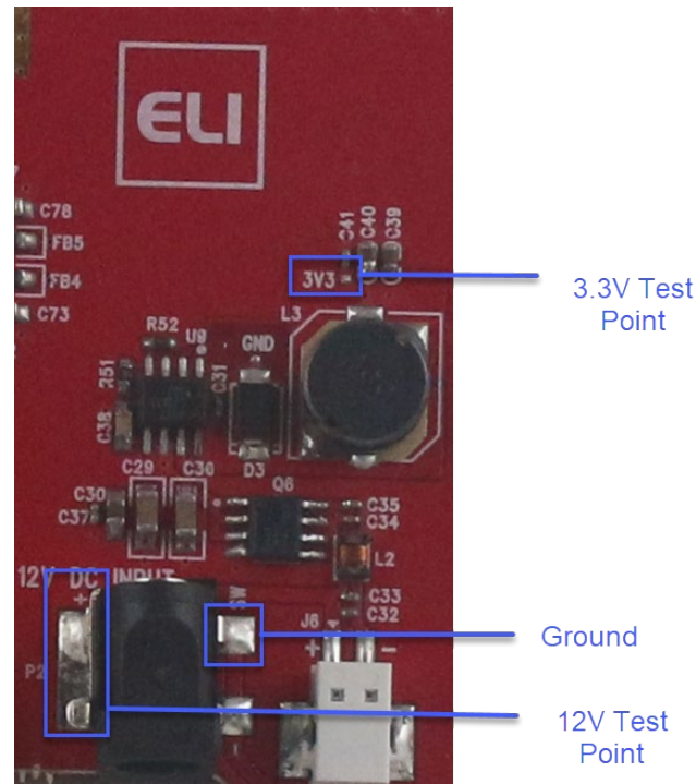
Figure 3. ELI70-CP Power Test Points
