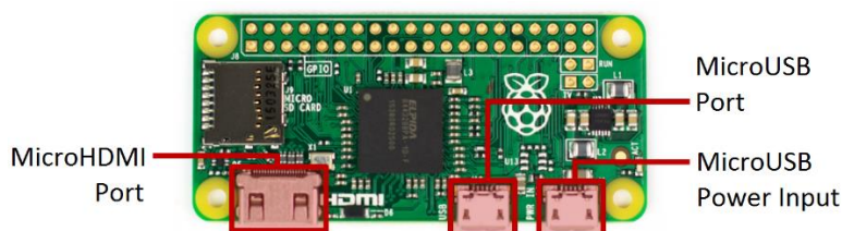
Figure 2. Raspberry Pi Zero Connections
