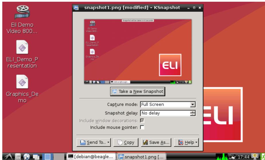
Figure 15. KSnapShot
