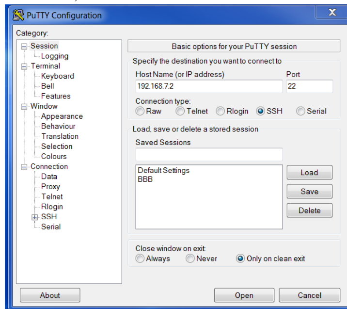
Figure 12. PuTTY Configuration
