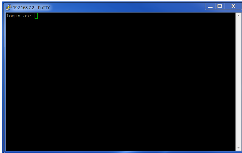
Figure 13. PuTTY Terminal
