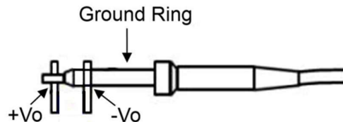
Single Models Dual Models Using Probe to Measure Output Ripple and Noise
