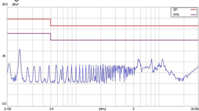
Figure18-1 EMI Conducted Class A for EC2SA11NH
