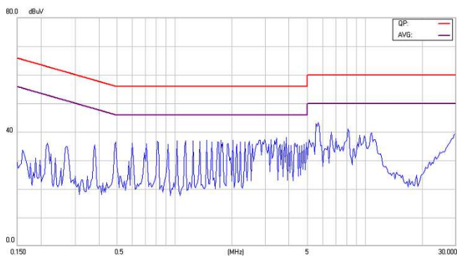
Figure16-2 EMI Conducted Class B for EC2SA05NH
