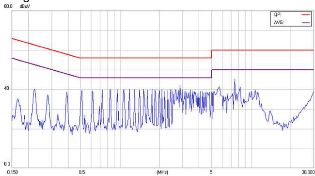
Figure19-2 EMI Conducted Class B for EC2SA12NH
