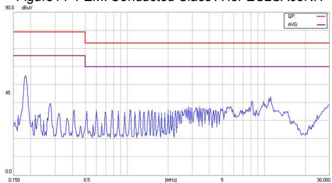
Figure15-1 EMI Conducted Class A for EC2SA04NH
