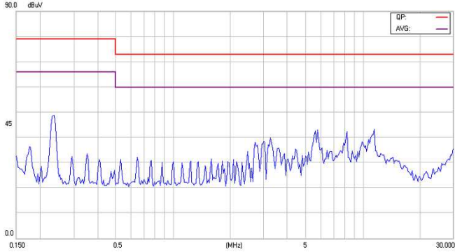
Figure22-1 EMI Conducted Class A for EC2SA15NH
