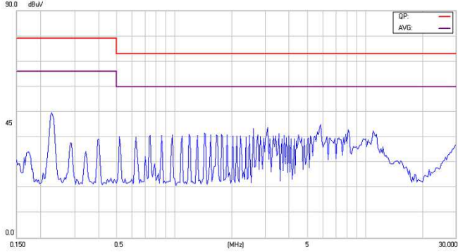
Figure21-1 EMI Conducted Class A for EC2SA14NH
