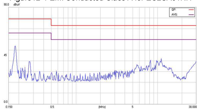
Figure13-1 EMI Conducted Class A for EC2SA02NH
