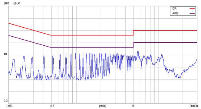
Figure20-2 EMI Conducted Class B for EC2SA13NH
