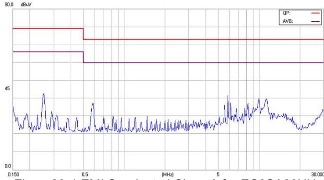
Figure29-1 EMI Conducted Class A for EC2SA26NH
