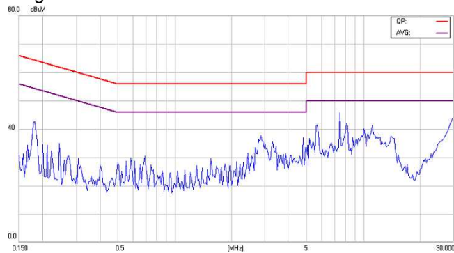
Figure13-2 EMI Conducted Class B for EC2SA02NH
