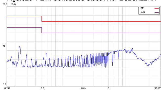
Figure26-1 EMI Conducted Class A for EC2SA23NH
