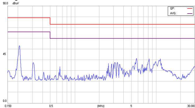
Figure23-1 EMI Conducted Class A for EC2SA16NH
