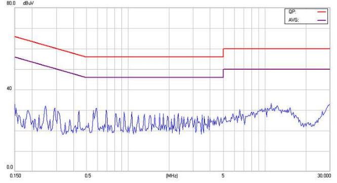
Figure29-2 EMI Conducted Class B for EC2SA26NH
