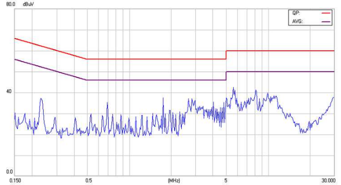
Figure22-2 EMI Conducted Class B for EC2SA15NH
