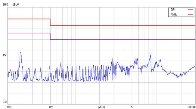
Figure16-1 EMI Conducted Class A for EC2SA05NH
