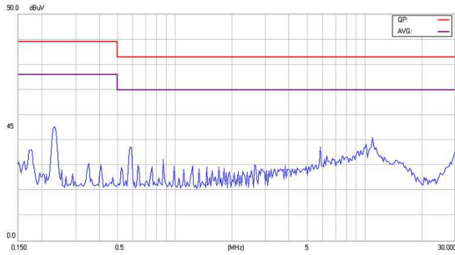
Figure28-1 EMI Conducted Class A for EC2SA25NH
