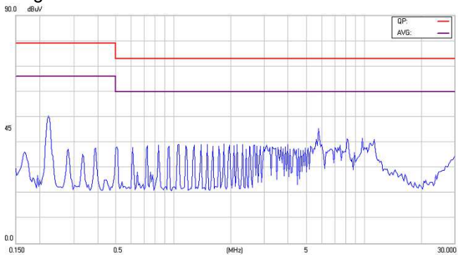
Figure19-1 EMI Conducted Class A for EC2SA12NH
