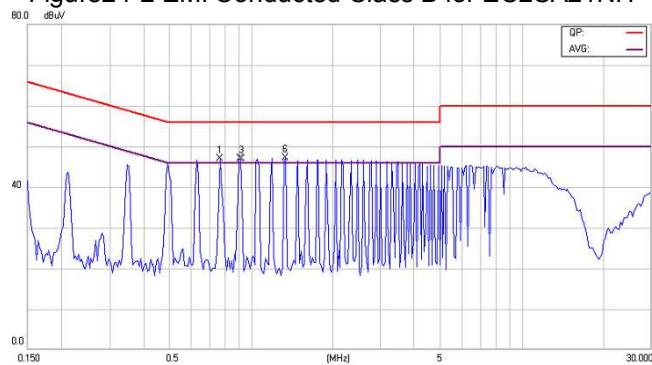
Figure25-2 EMI Conducted Class B for EC2SA22NH
