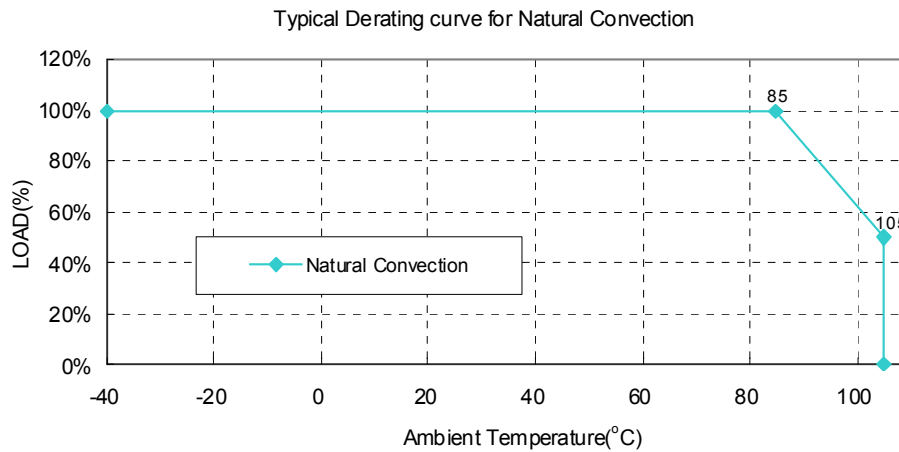
Figure4 Typical Power De-rating Curve for EC2SANH Series
