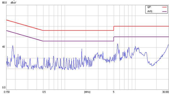
Figure17-2 EMI Conducted Class B for EC2SA06NH
