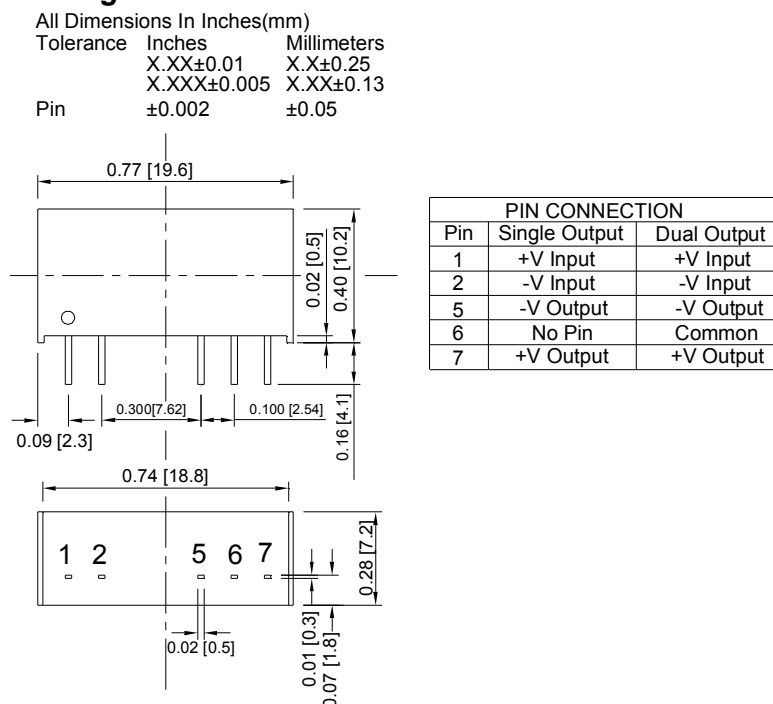
Figure30 EC2SANH Mechanical Outline Diagram
