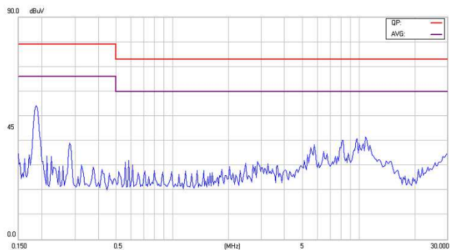
Figure12-1 EMI Conducted Class A for EC2SA01NH
