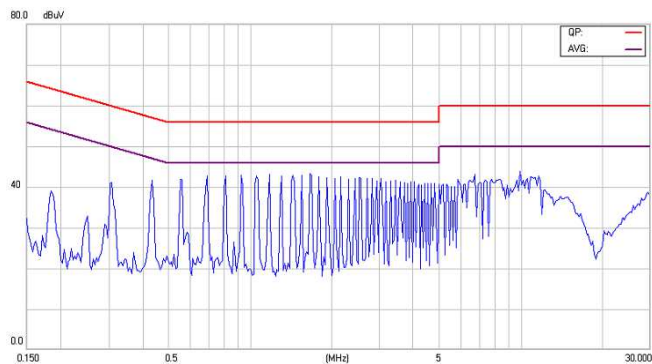
Figure24-2 EMI Conducted Class B for EC2SA21NH
