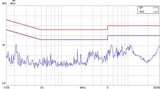
Figure14-2 EMI Conducted Class B for EC2SA03NH
