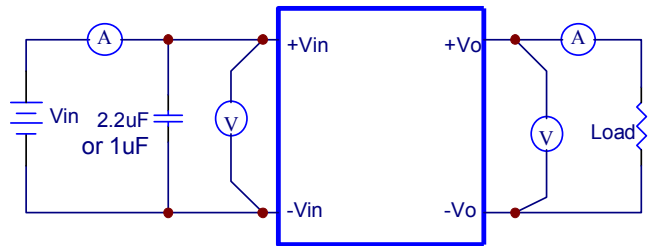
Figure6 EC2SANH Series Single output Test Setup
