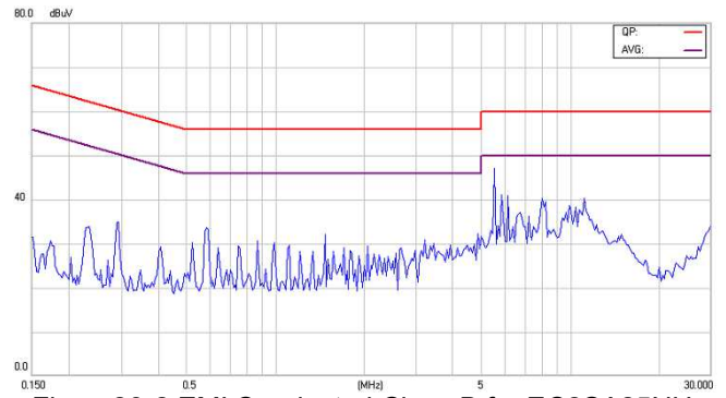
Figure28-2 EMI Conducted Class B for EC2SA25NH
