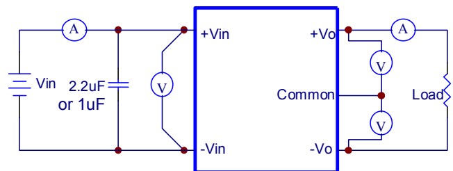
Figure7 EC2SANH Series Dual output Test Setup
