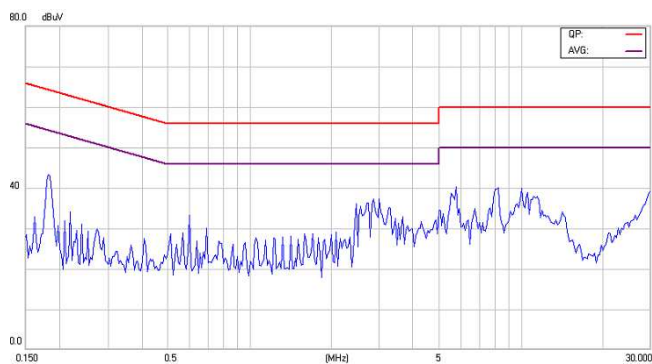
Figure12-2 EMI Conducted Class B for EC2SA01NH
