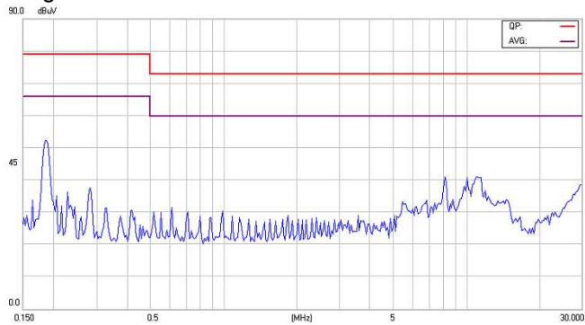
Figure17-1 EMI Conducted Class A for EC2SA06NH
