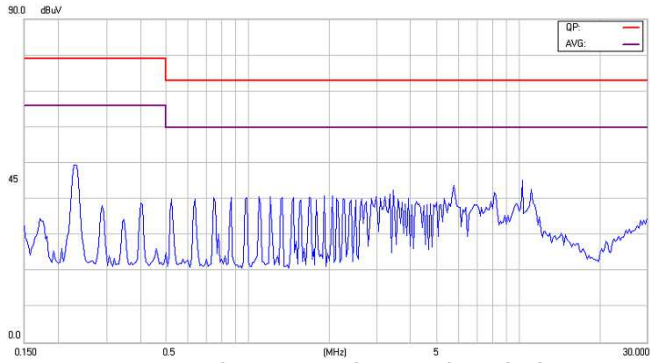
Figure20-1 EMI Conducted Class A for EC2SA13NH
