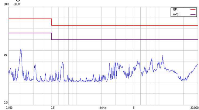
Figure14-1 EMI Conducted Class A for EC2SA03NH
