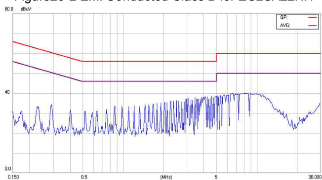
Figure26-2 EMI Conducted Class B for EC2SA23NH
