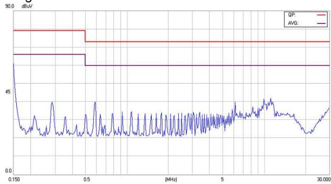
Figure27-1 EMI Conducted Class A for EC2SA24NH
