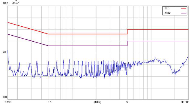
Figure27-2 EMI Conducted Class B for EC2SA24NH
