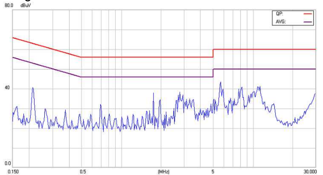
Figure23-2 EMI Conducted Class B for EC2SA16NH
