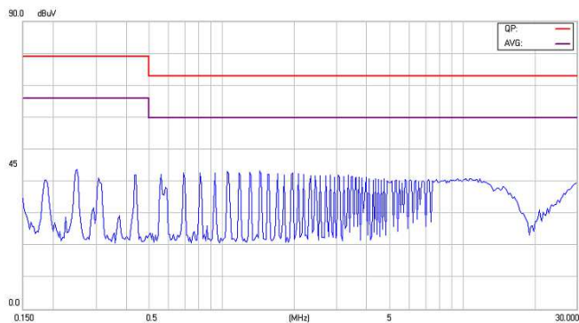
Figure24-1 EMI Conducted Class A for EC2SA21NH
