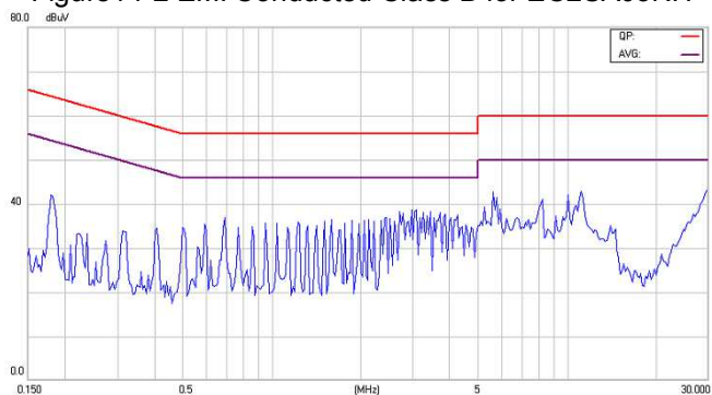
Figure15-2 EMI Conducted Class B for EC2SA04NH
