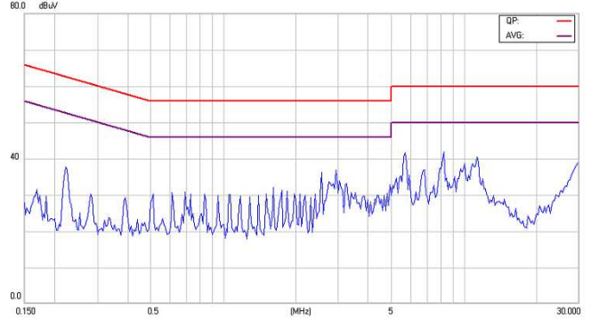
Figure21-2 EMI Conducted Class B for EC2SA14NH
