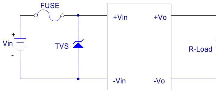
Figure10 Input Protection
