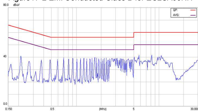
Figure18-2 EMI Conducted Class B for EC2SA11NH
