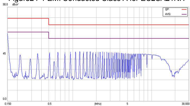
Figure25-1 EMI Conducted Class A for EC2SA22NH
