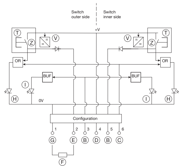
Wiring diagram 2
