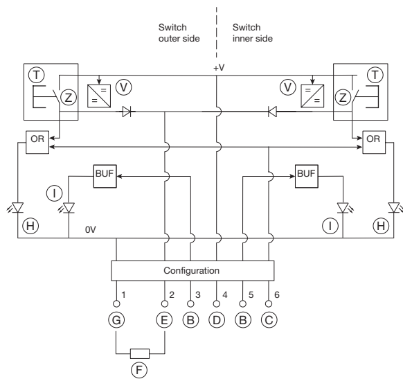
Wiring diagram 1
