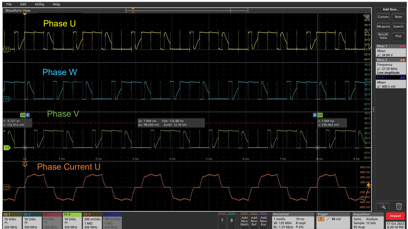
Figure 5: Example of 120 Degree (Trapezoidal) commutation
