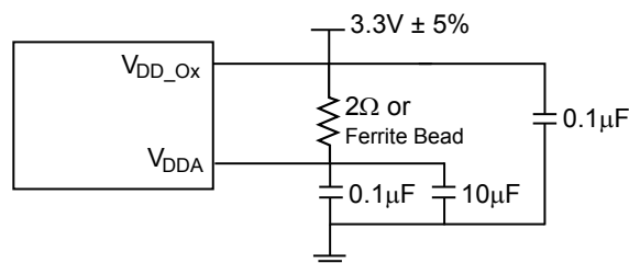
Figure 4. Power Supply Filter
