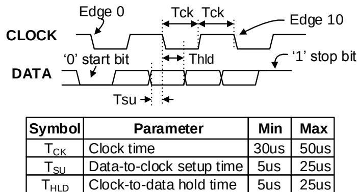
Figure 11. PS/2 Device-to-Host Timing Diagram.
