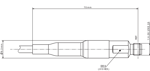
2.92 mm female (SF_21_SK-503)
