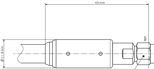
2.92 mm male (SF_11_SK-504)
