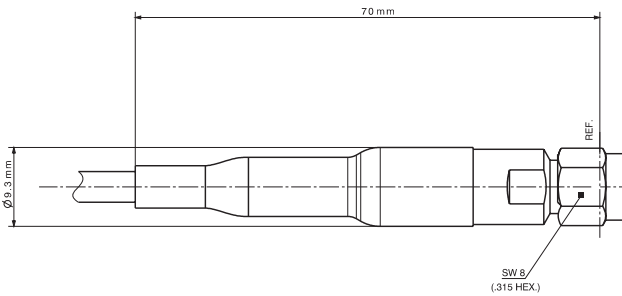
2.92 mm male (SF_11_SK-502)
