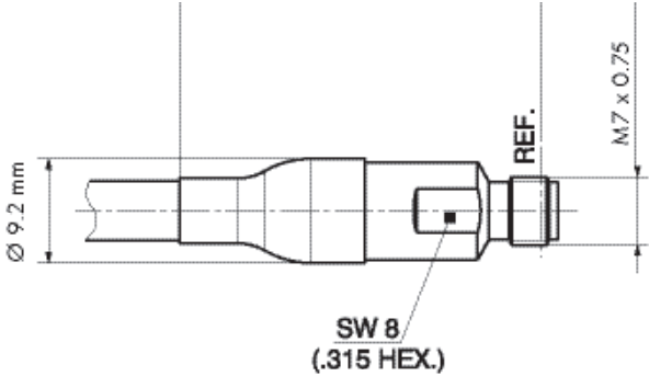
2.4 mm female (SF_21_PC24-501)
