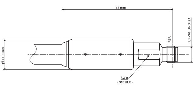
2.92 mm female (SF_21_SK-504)
