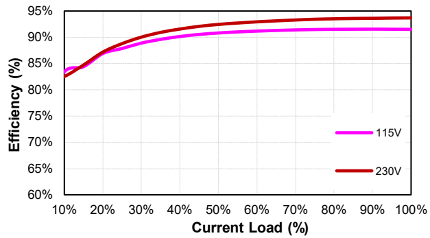
LFM300S300 (Eff Vs Io)
