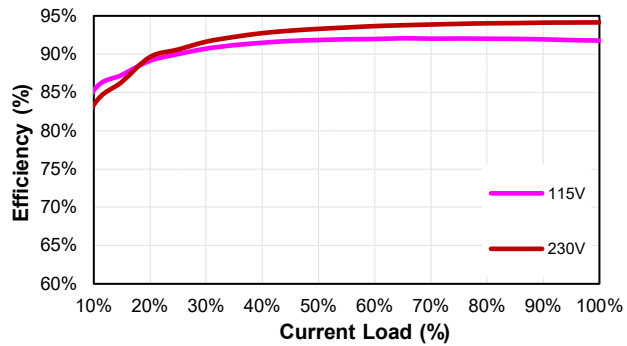
LFM300S540 (Eff Vs Io)
