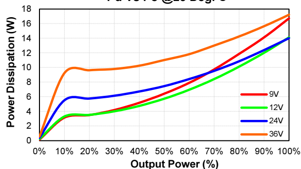
CQB150W-24S15 Pd Vs Po @25 Deg. C
