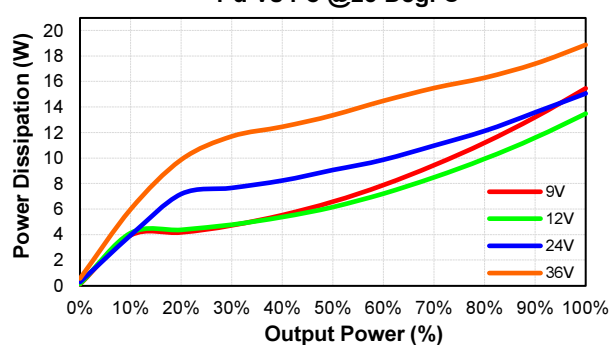
CQB150W-24S24 Pd Vs Po @25 Deg. C
