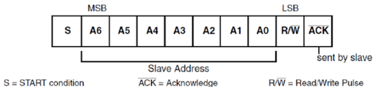
Figure 13 7-bit Address Format
