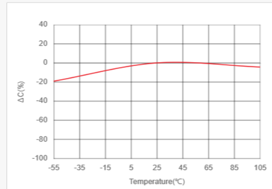
Temperature Characteristics of Capacitance(TCC) LCR meter, 0.12kHz, 0.15Vrms
