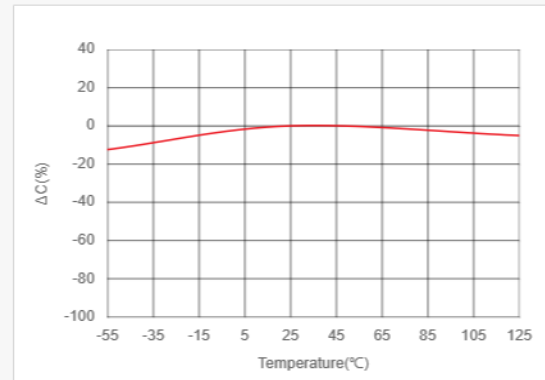
Temperature Characteristics of Capacitance(TCC) LCR meter, 1kHz, 0.4Vrms
