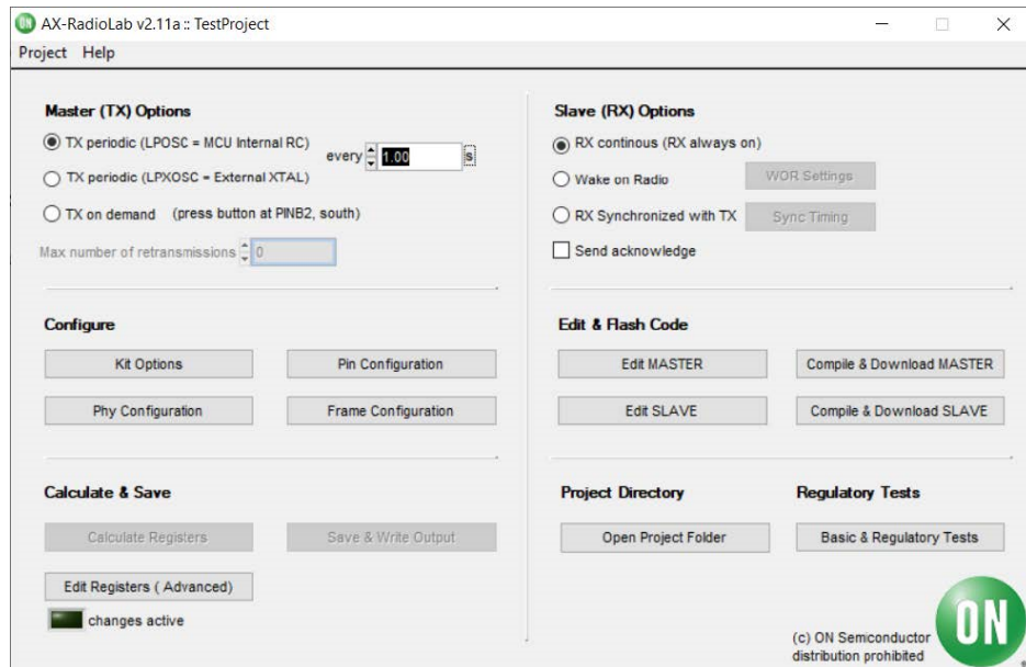
Figure 10. Screenshot of AX-RadioLab Main Panel GUI
