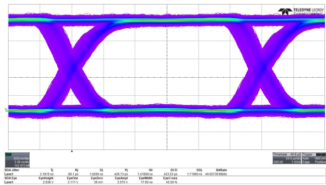
Figure 30. Receiver output. Eye diagram @ V_{CC} = 3.3\text{ V} data rate 50 Mbps, d = 1\text{ m}
