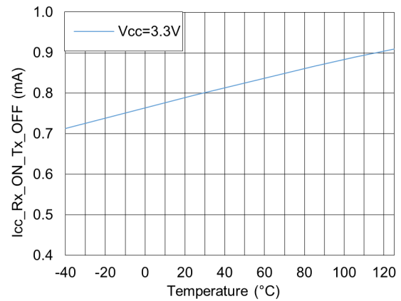
Figure 16. No-load supply current vs. temperature, DE = GND, RE = GND @ V CC = 3.3 V
