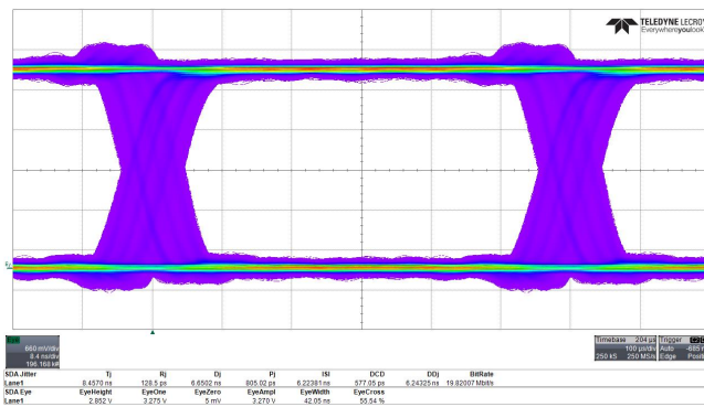
Figure 29. Receiver output. Eye diagram @ V_{CC} = 3.3\text{ V} , Data rate 20 Mbps, d = 100\text{ m}
