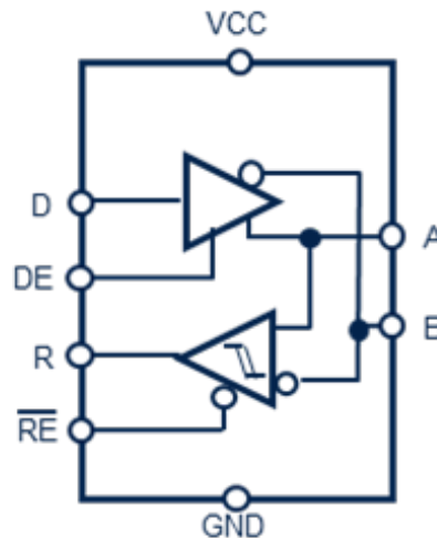
Figure 31. Block diagram
