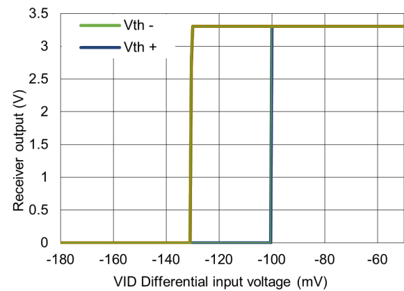
Figure 28. Receiver output vs. input @ V_{CC} = 3.3\text{ V}
