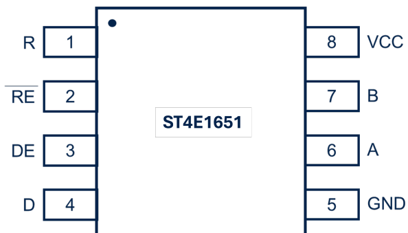
Figure 1. Pin connections
