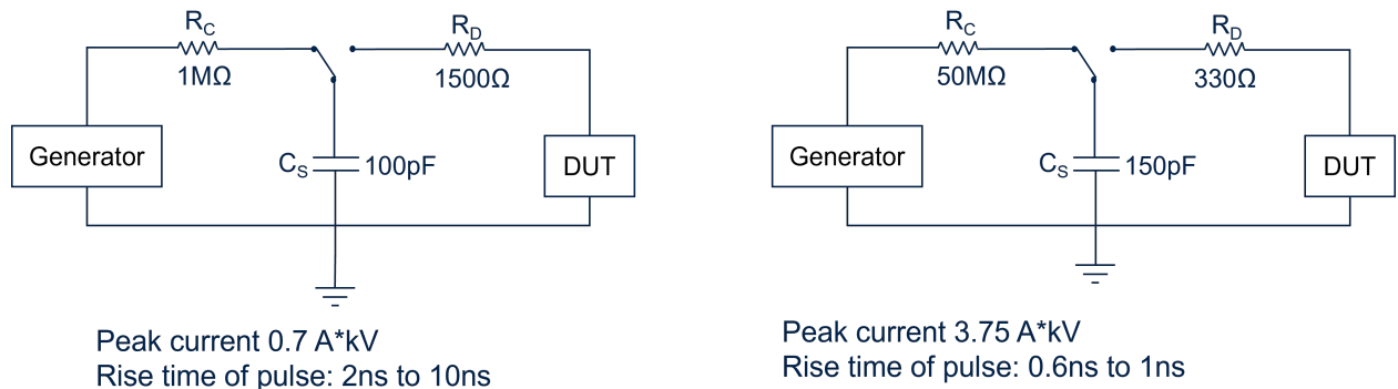
Figure 33. HBM JEDEC (left) and IEC61000-4-2 (right) generator simplified schematics
