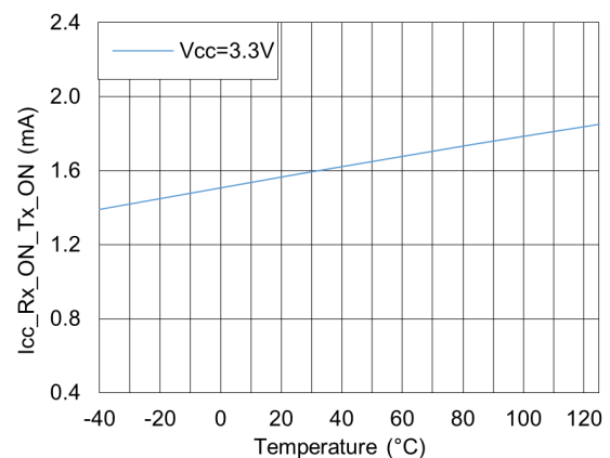
Figure 18. No-load supply current vs. temperature, DE = V CC , RE = GND @ V CC = 3.3 V
