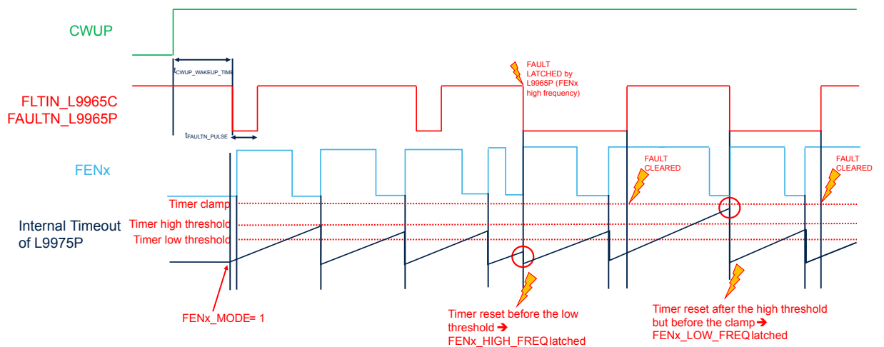
Figure 12. FENx line integrity check in PWM mode (example of frequency out of range)
