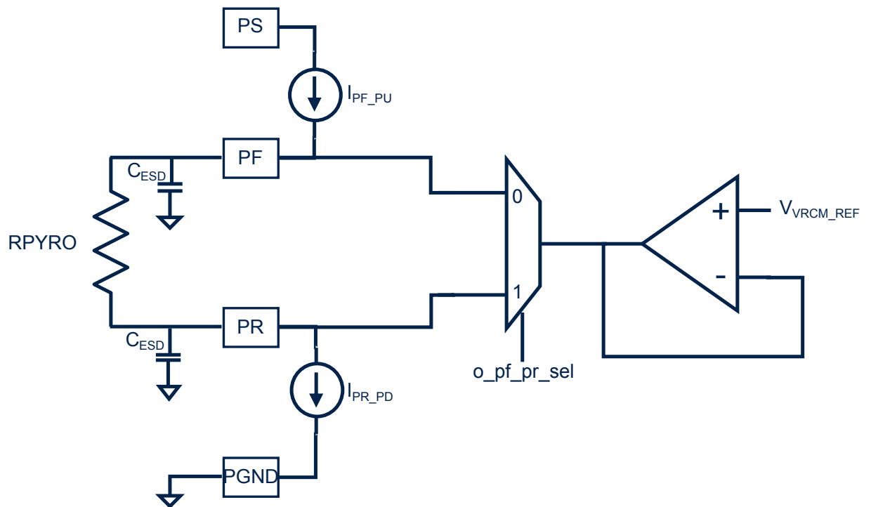
Figure 20. VRCM test
