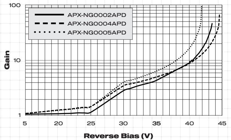
Typical Gain vs. Reverse Voltage at 1550nm
