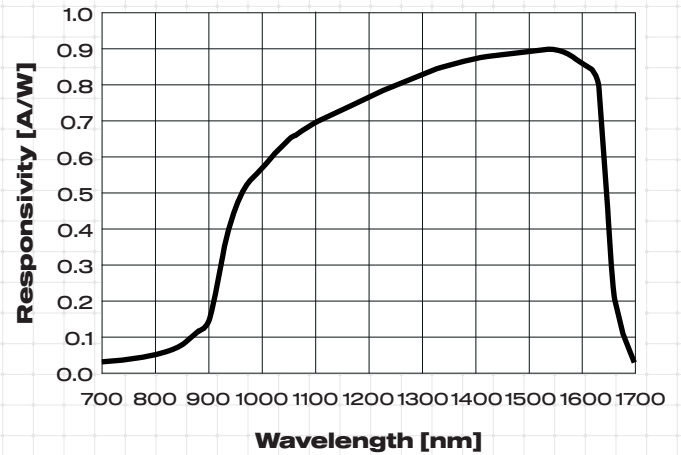
Typical Spectral Response at M=1
