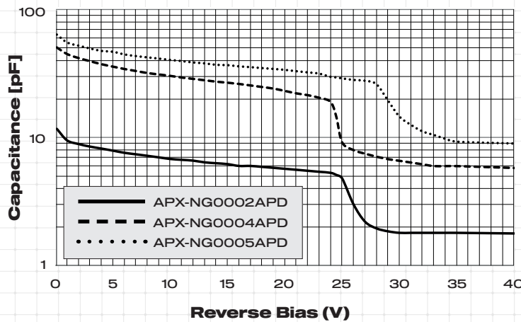
Typical Capacitance vs. Reverse Voltage
