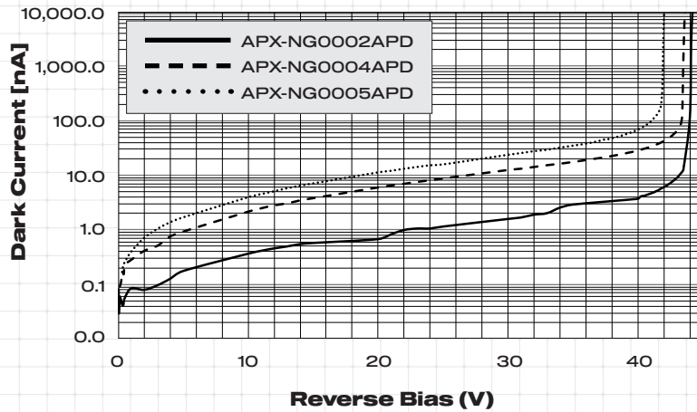
Typical Dark Current vs. Reverse Voltage
