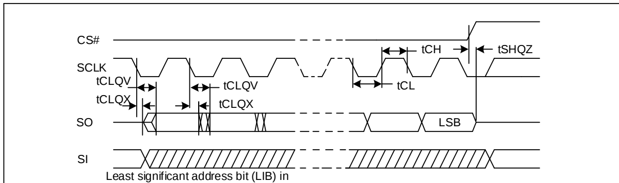
Figure 24-2. Output Timing
