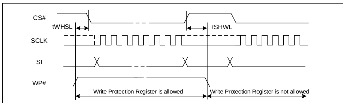
Figure 24-7. WP# Timing
