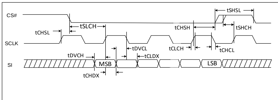
Figure 24-3. Serial Input Timing (DTR)
