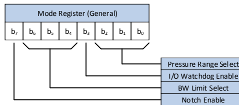
Mode Control Register Detail
