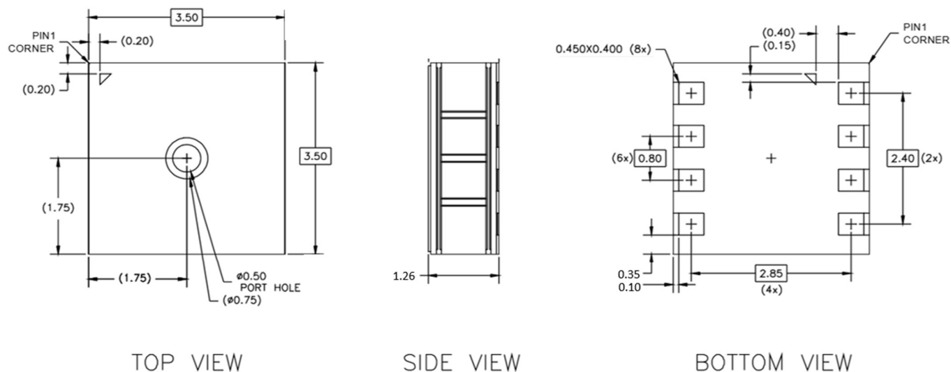
Figure 6. CH-101 Dimensions
