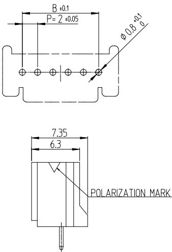
Recommended PCB Layout (t=1.6mm)
