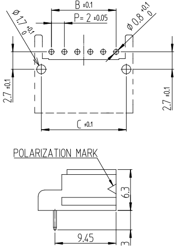
Recommended PCB Layout (t=1.6mm)
