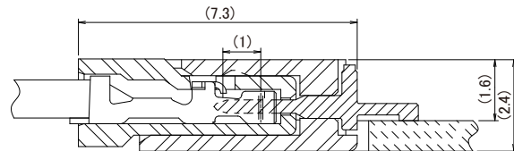
DF14H Offset Type Board Mounted Diagram
