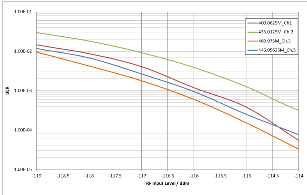
Figure 38 DE9941A-435 Rx Sensitivity at Different Frequencies with 4-FSK, 4.8 ksybols/s
