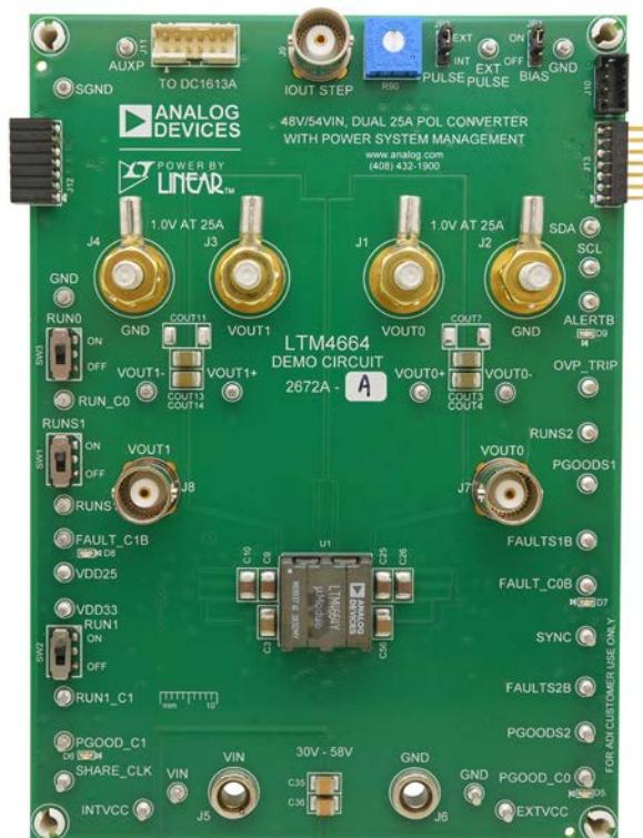
Figure 1. Dual-output LTM4664/DC2672A-A Demo Circuit
