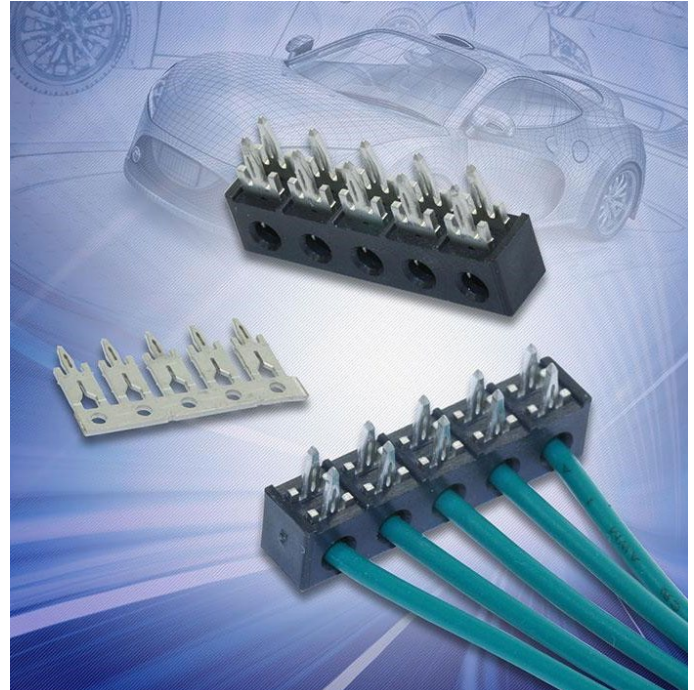
Figure 4 AVX Press-Fit IDC 53-8702
