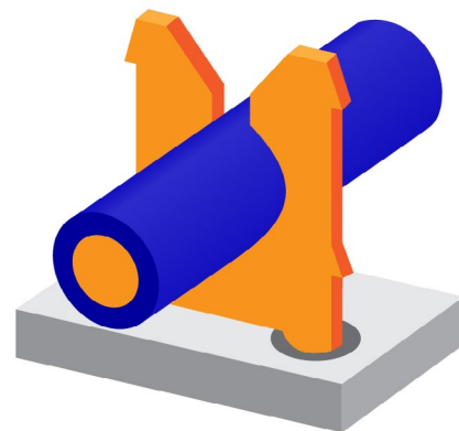
Figure 2 Insulation Displacement Connection [AVX.com]
