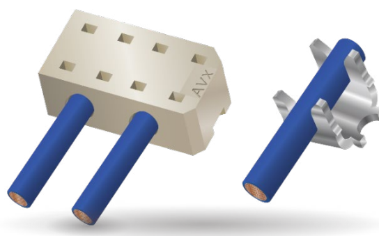
Figure 3 AVX Low Profile IDC Connector
