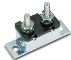
30055-30 12V 30A Type 1 Boxed Style Circuit Breaker
