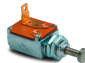
91812 12V 5A Normally Closed Self Grounded Door Switch
