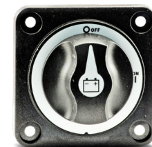
880062 SR Series Panel Mount Disconnect Switch
