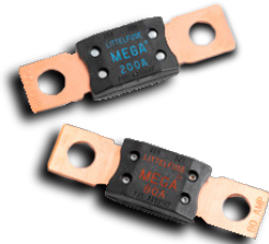
MEGA® FUSES 80A - 500A
