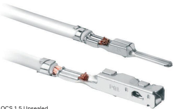
OCS 1.5 Unsealed Female & Male Terminals
