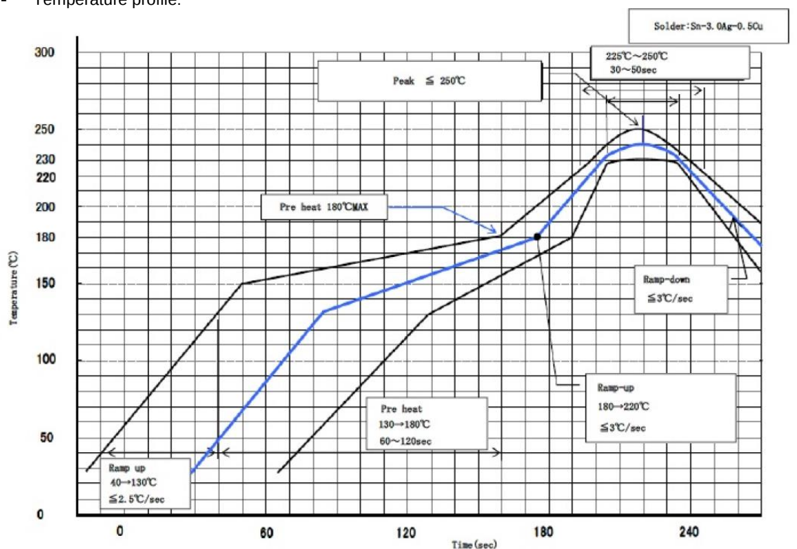
Figure 19: Temperature profile
