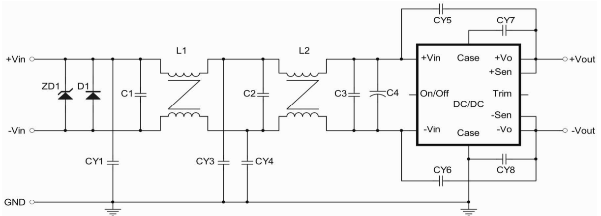
Figure1 Connection circuit
