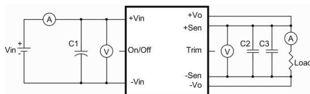
CQB75W8 Series Test Setup
