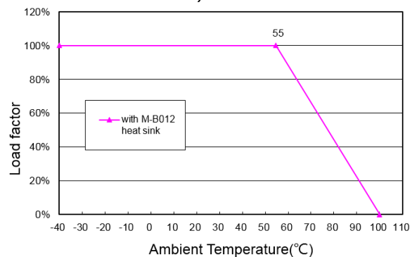
Ambient Derating Curves at Nominal Line, Full Load and Natural Convection
