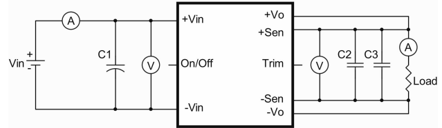
CQB100W8 Series Test Setup
